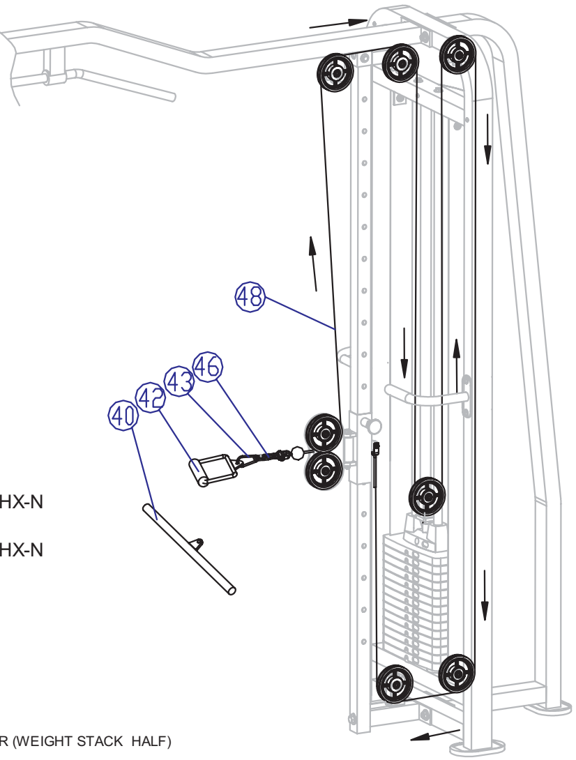
CABLE ROUTING DETAIL
